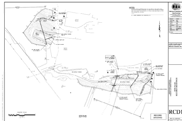
Dry Swale
