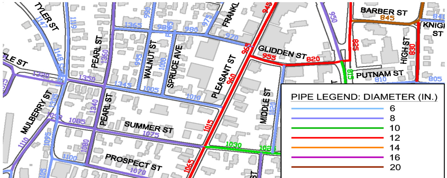
Water System Model Schematic
